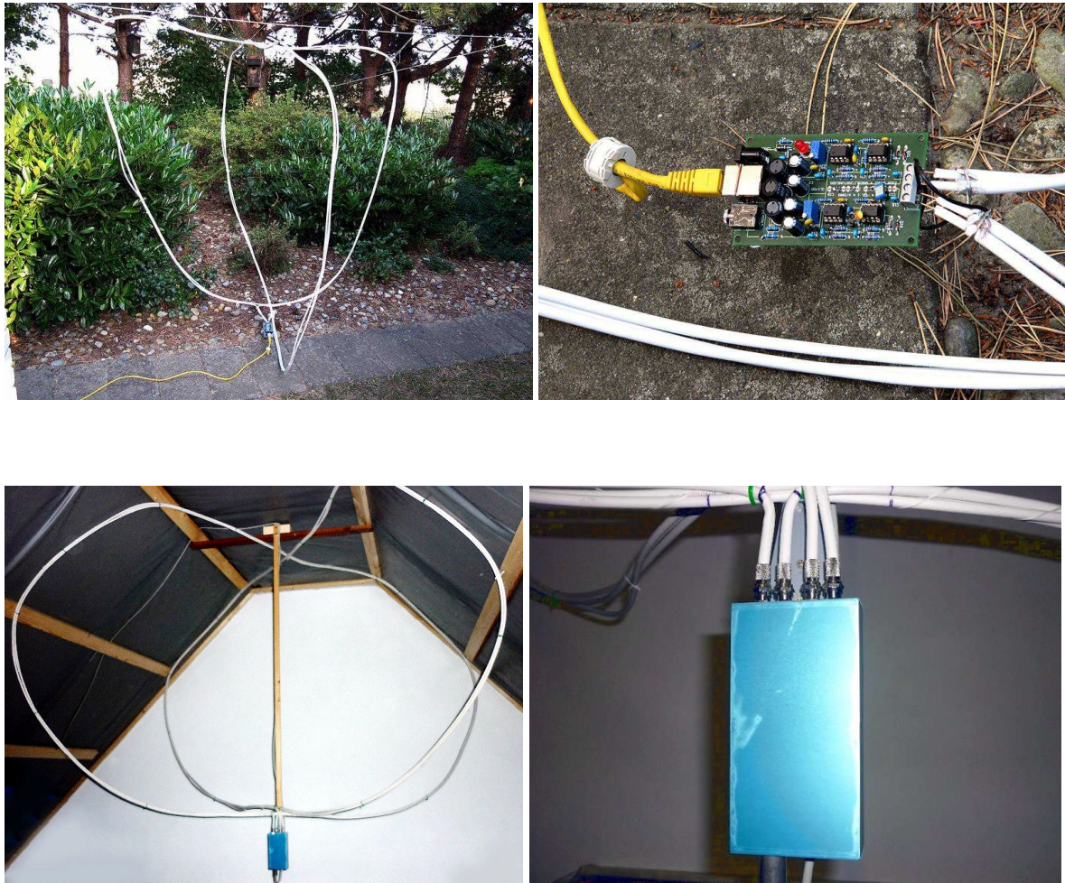
Figure 18: Connecting a coax antenna, ©Richo Andersen and Bernhard Kilimann
