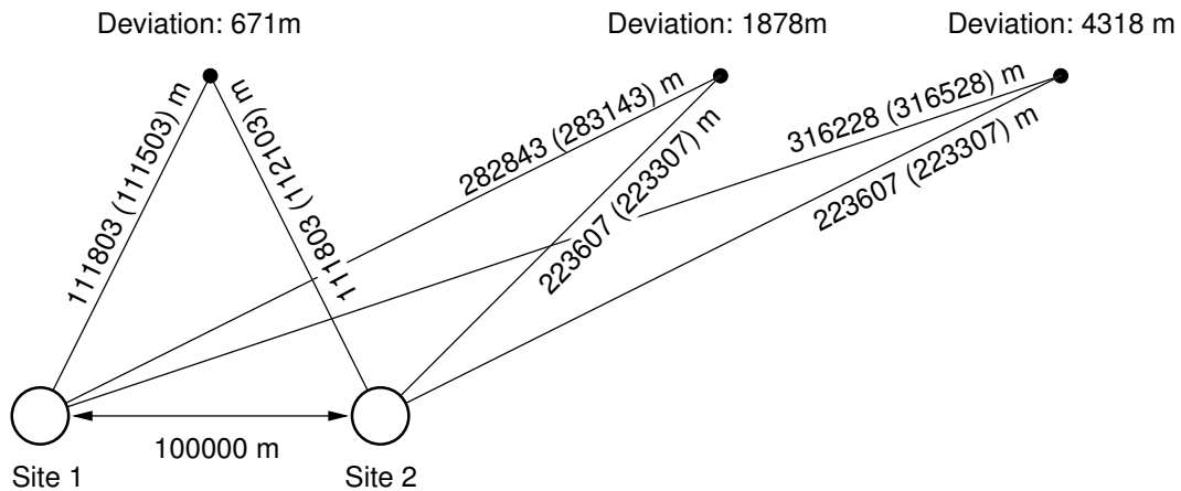
Figure 8: The deviations for an accuracy of \pm 1 \mu s for different cut angles
