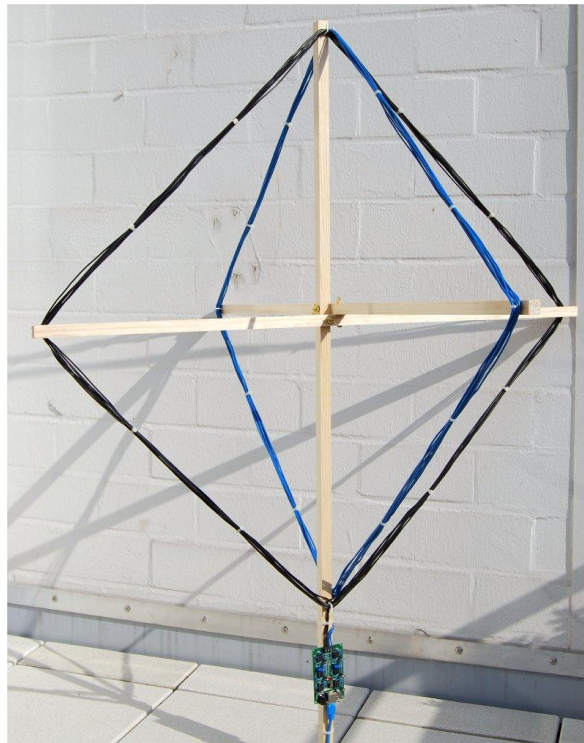
Figure 3: Two orthogonal crossed VLF loop antennas, 8 turns, diagonal size 1 m connected to amplifier PCB 3 Version 2.
