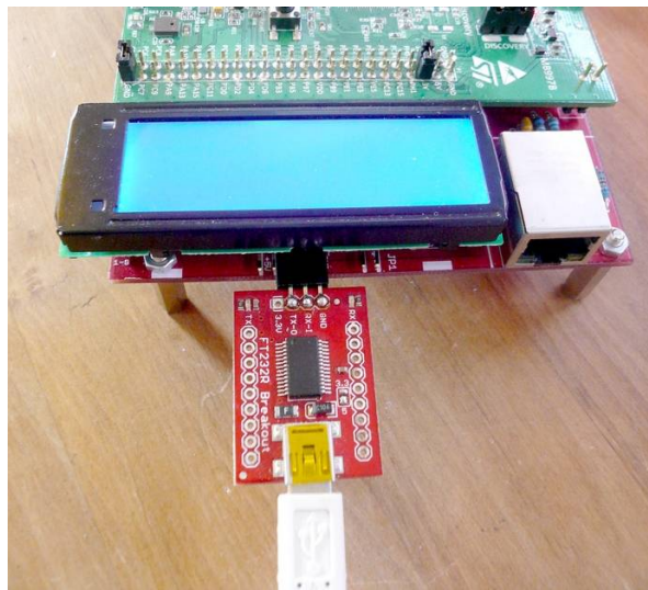
Figure 46: A serial-to-USB adapter connected to the controller
