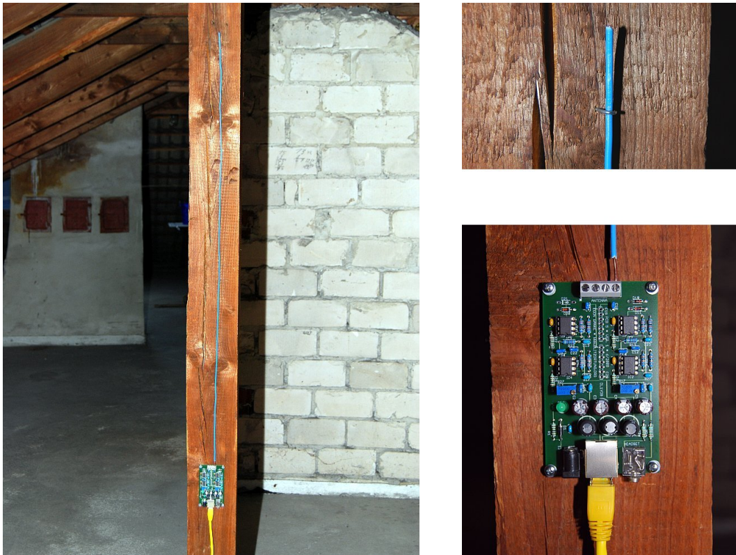
Figure 24: A wire of 1 meter length used as an electrical antenna connected to an old amplifier PCB 5 Version 1
