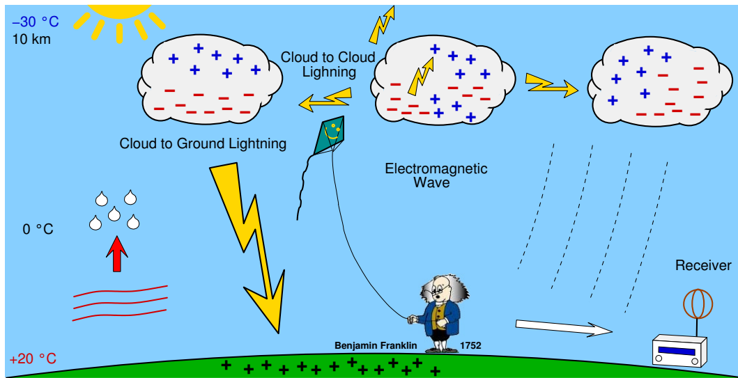
Figure 2: How lightning forms
