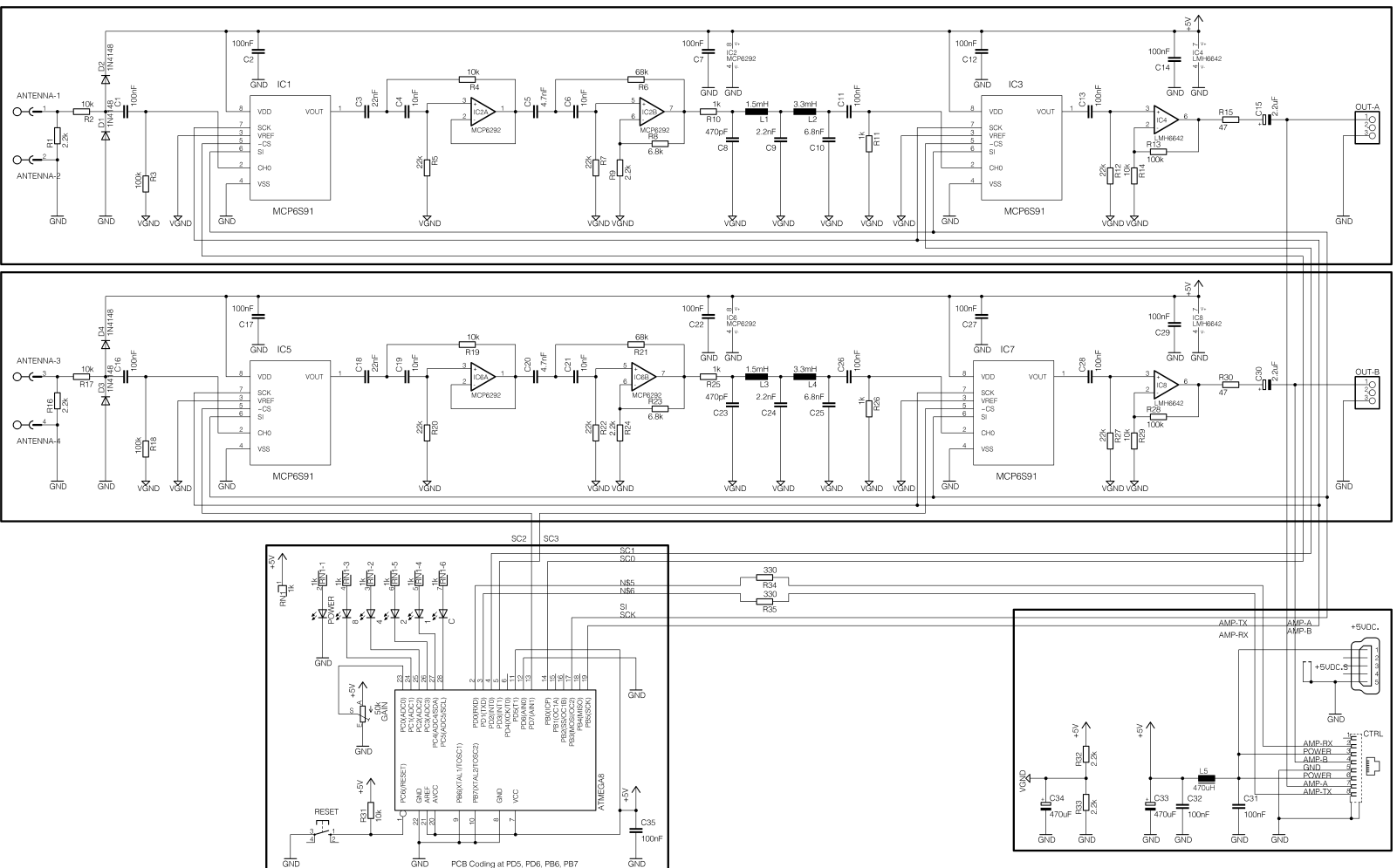
Figure 27: The complete circuit diagram of Amplifier 12.3
