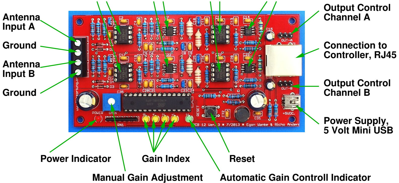
Figure 30: An assembled Amplifier 12 Version 3
