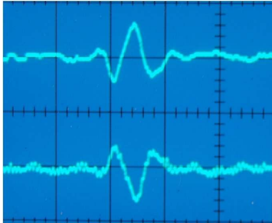
Figure 25: A signal of a lightning discharge received by an electrical antenna (above) and by a ferrite rod antenna (below)
