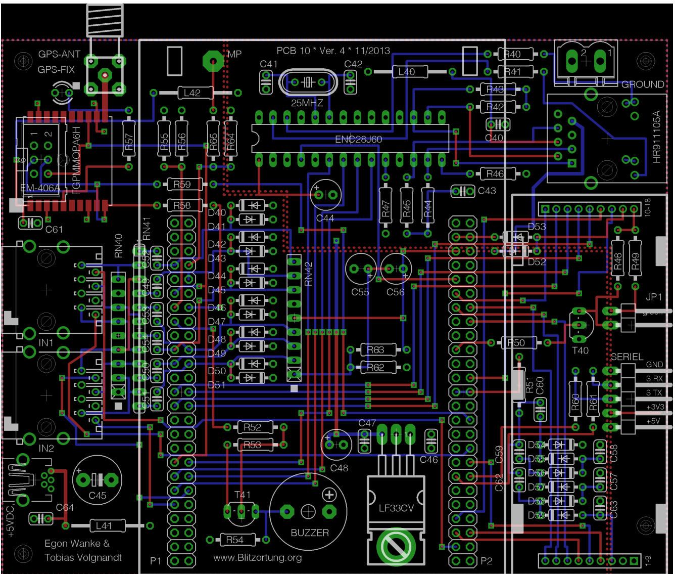
Figure 33: Printed Circuit Board of Controller 10.4
