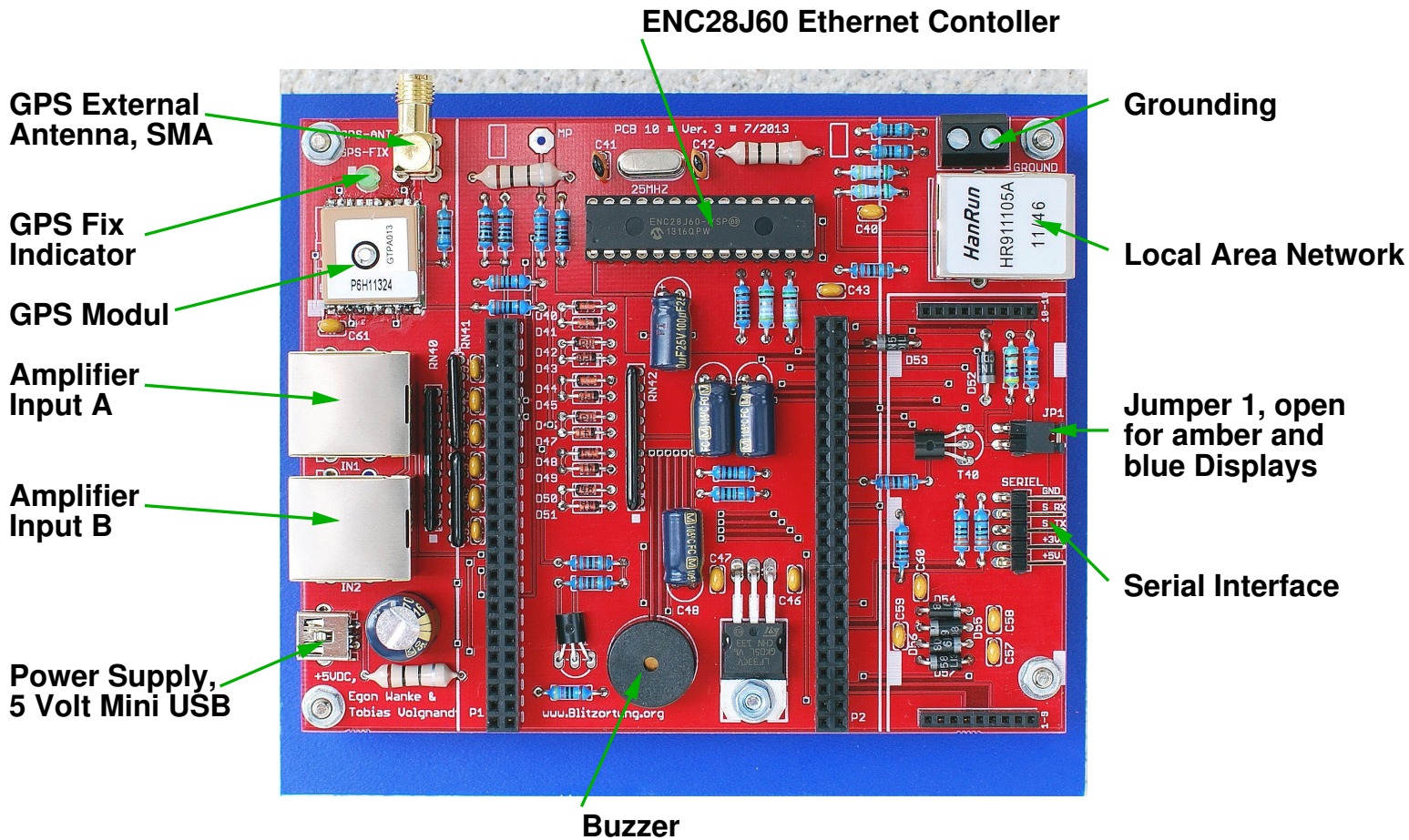
Figure 35: Assembled Controller 10.3
