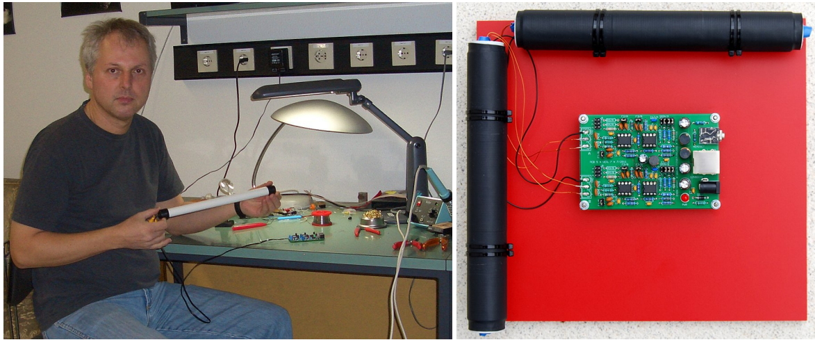
Figure 20: Egon holds a 35 cm ferrite rod antenna. Two 20 cm ferrite rod antennas mounted on a PVC board connected to amplifier PCB 5 Version 7
