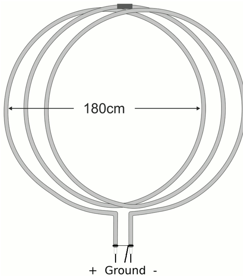
Figure 16: A coax antenna, ©Richo Andersen
