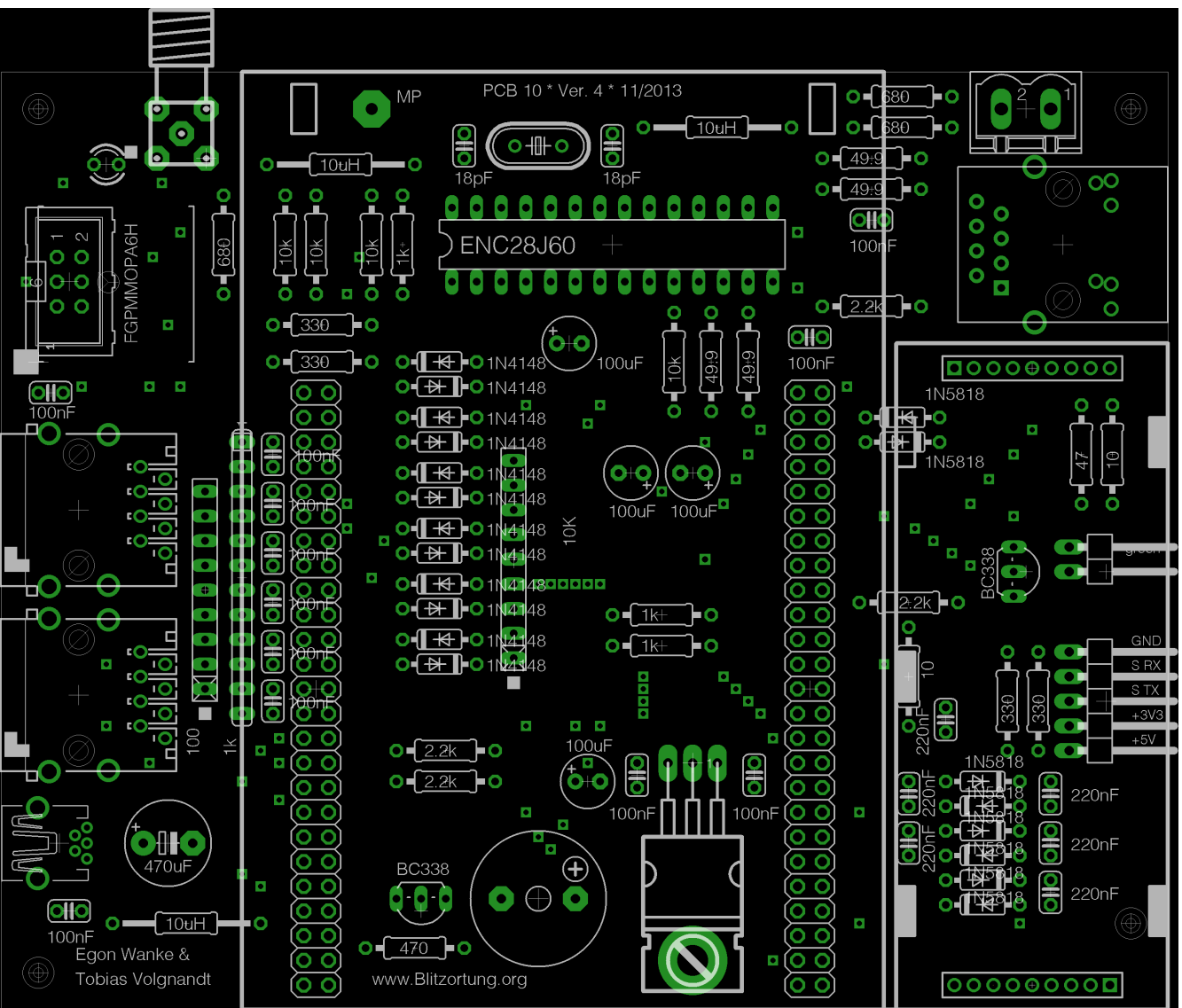
Figure 34: Assembly Diagram of Controller 10.4
