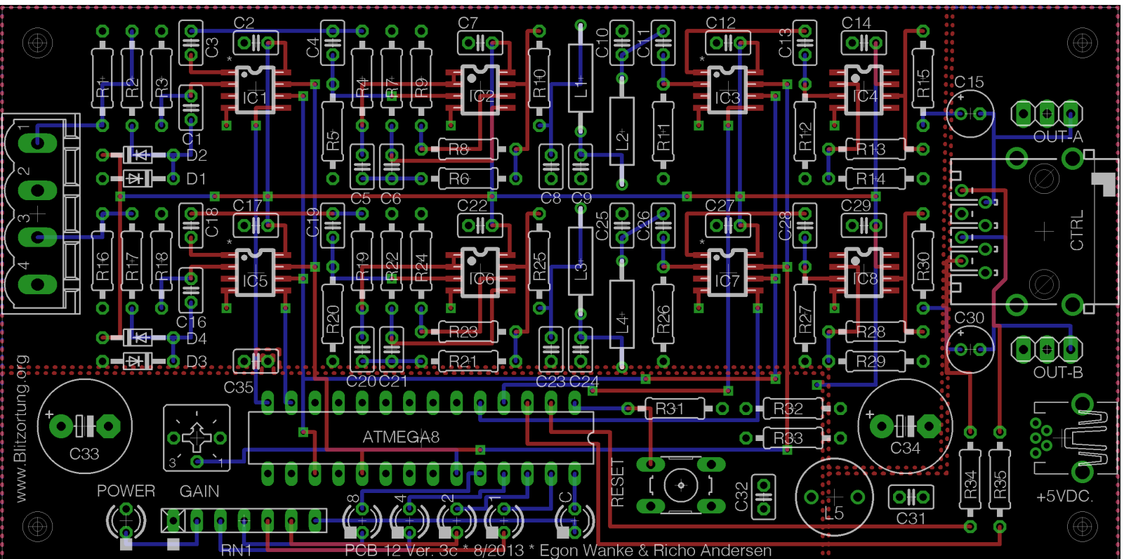
Figure 28: The Printed Circuit Board of Amplifier 12.3
