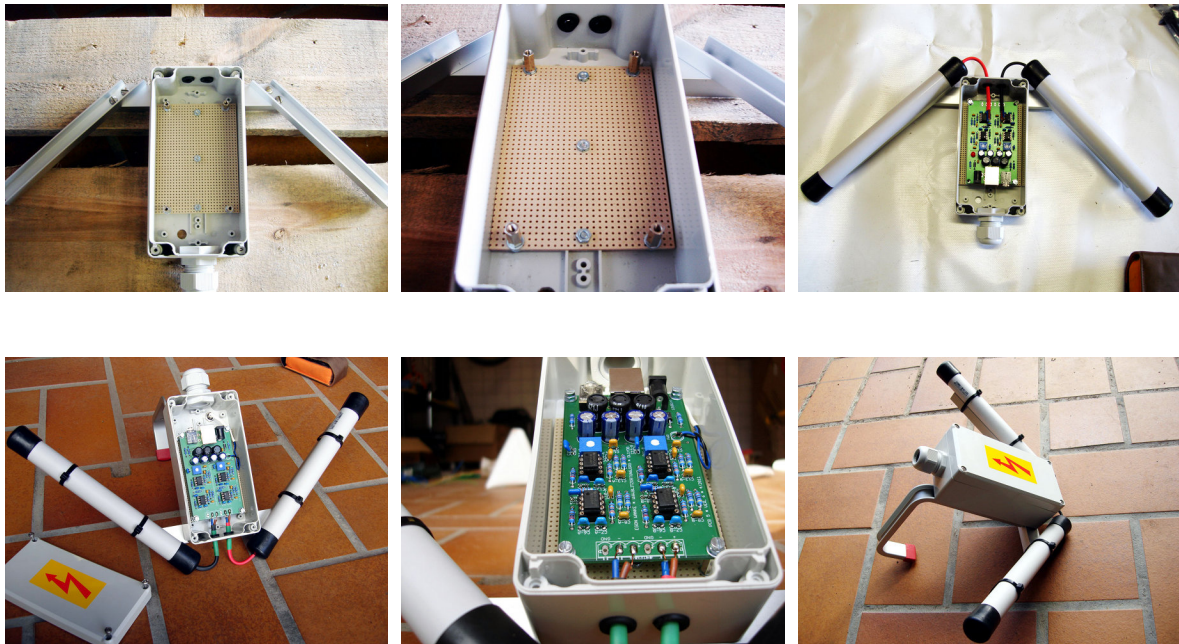
Figure 23: A guidance for building an outdoor ferrite rod antenna, continued, ©Florian Bamberg
