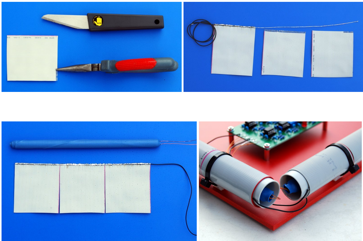
Figure 21: Shielding a ferrite rod antenna with ribbon cable
